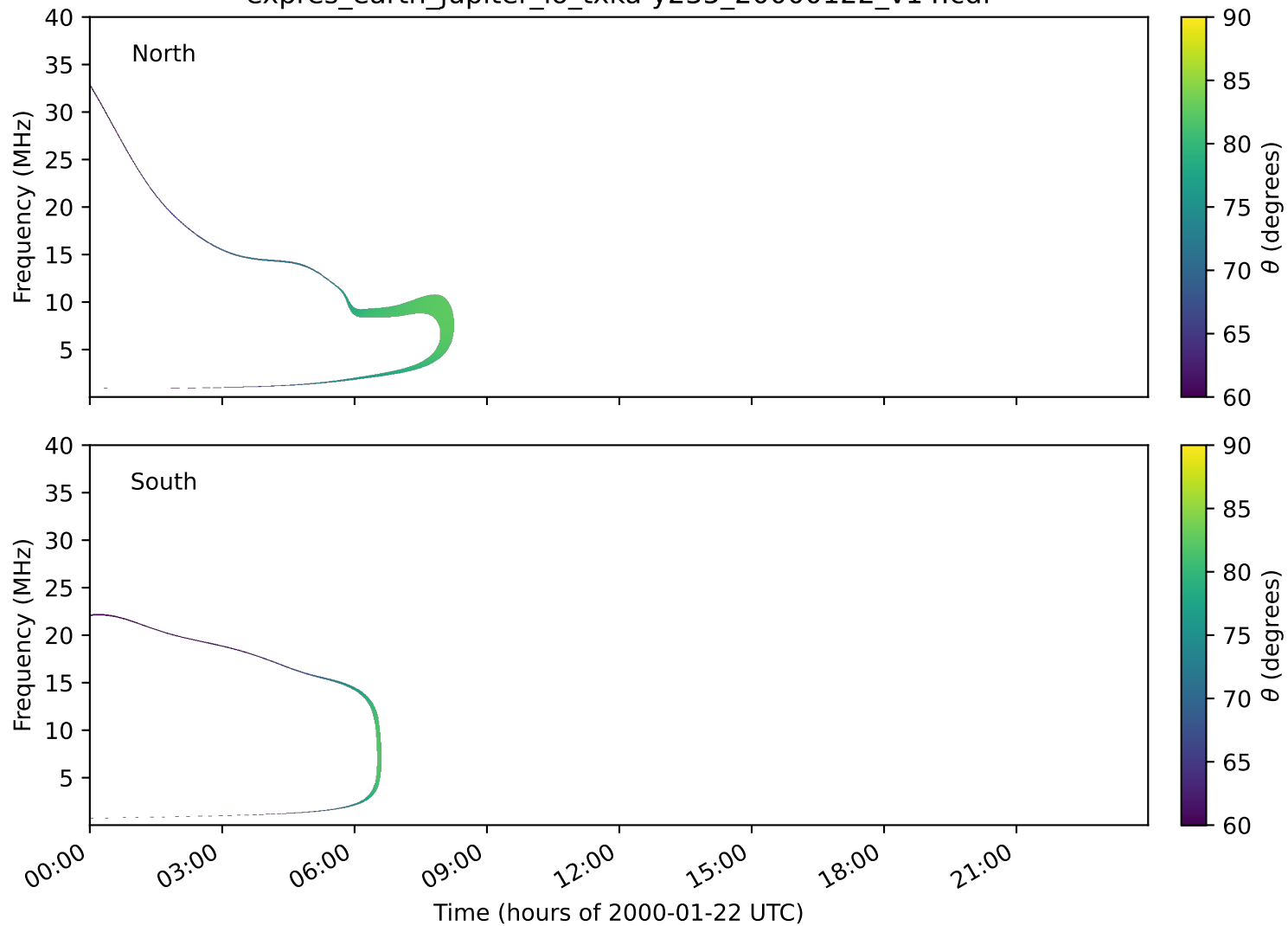
expres_earth_jupiter_io_txka-y235_20000122_v14.cdf
