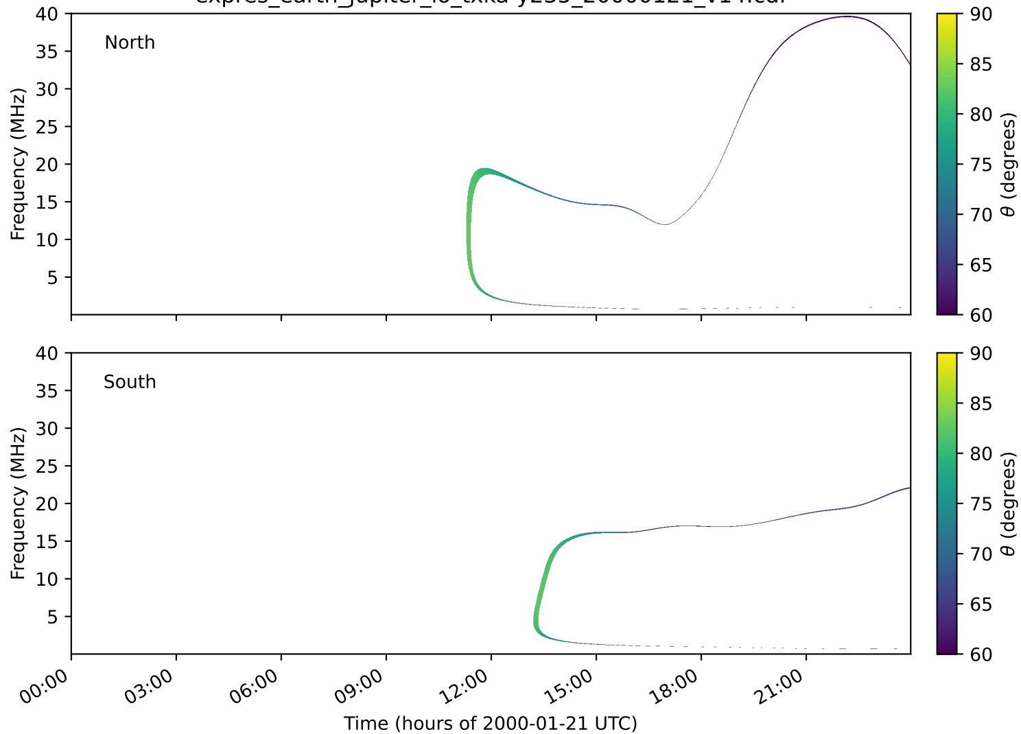
expres_earth_jupiter_io_txka-y235_20000121_v14.cdf
