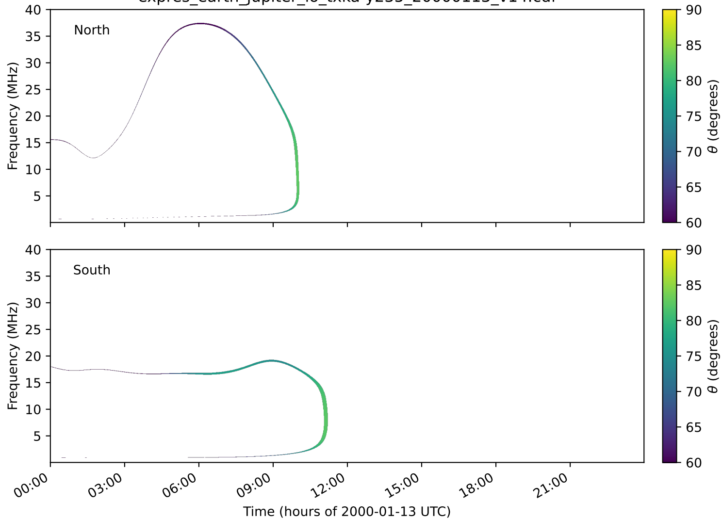
expres_earth_jupiter_io_txka-y235_20000113_v14.cdf
