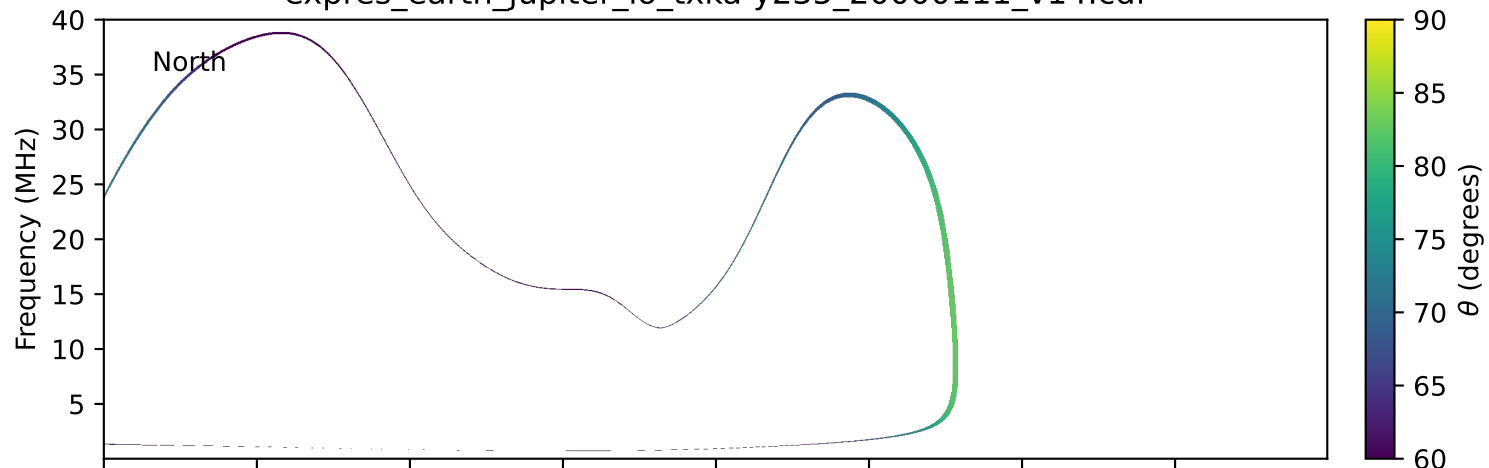
expres_earth_jupiter_io_txka-y235_20000111_v14.cdf
