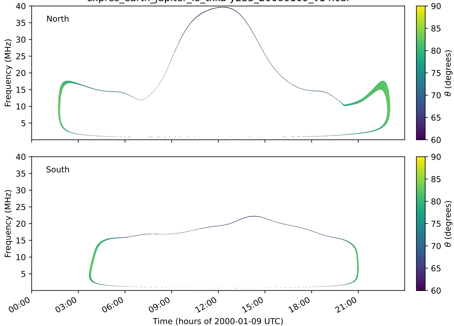
expres_earth_jupiter_io_txka-y235_20000109_v14.cdf
