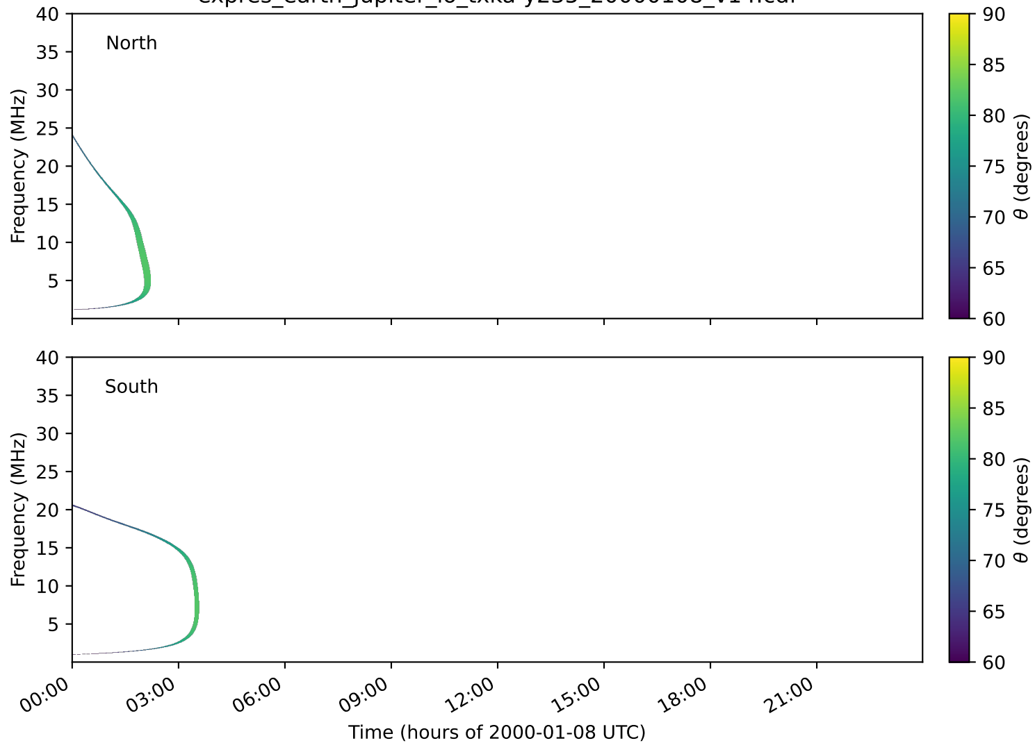
expres_earth_jupiter_io_txka-y235_20000108_v14.cdf
