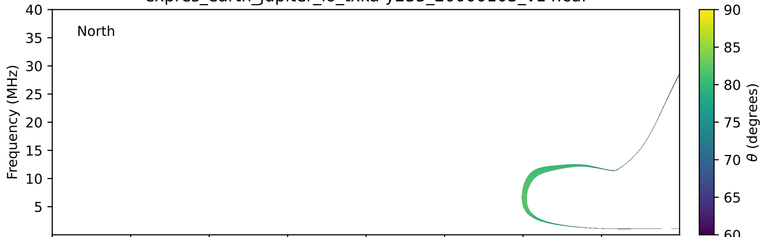
expres_earth_jupiter_io_txka-y235_20000103_v14.cdf
