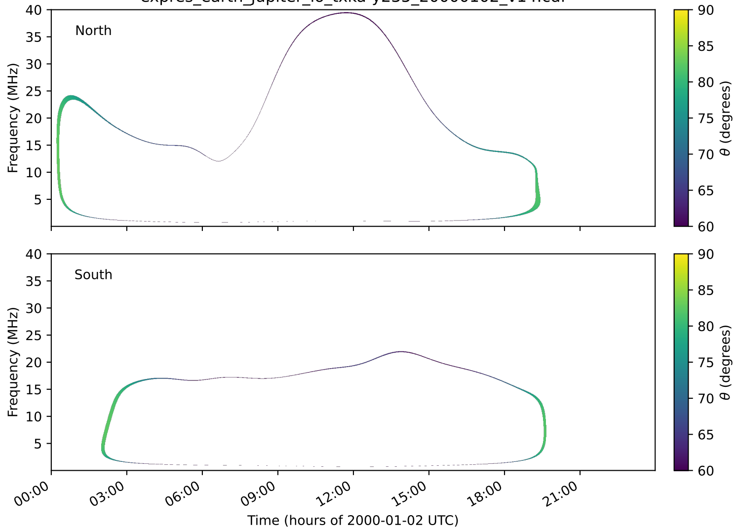
expres_earth_jupiter_io_txka-y235_20000102_v14.cdf
