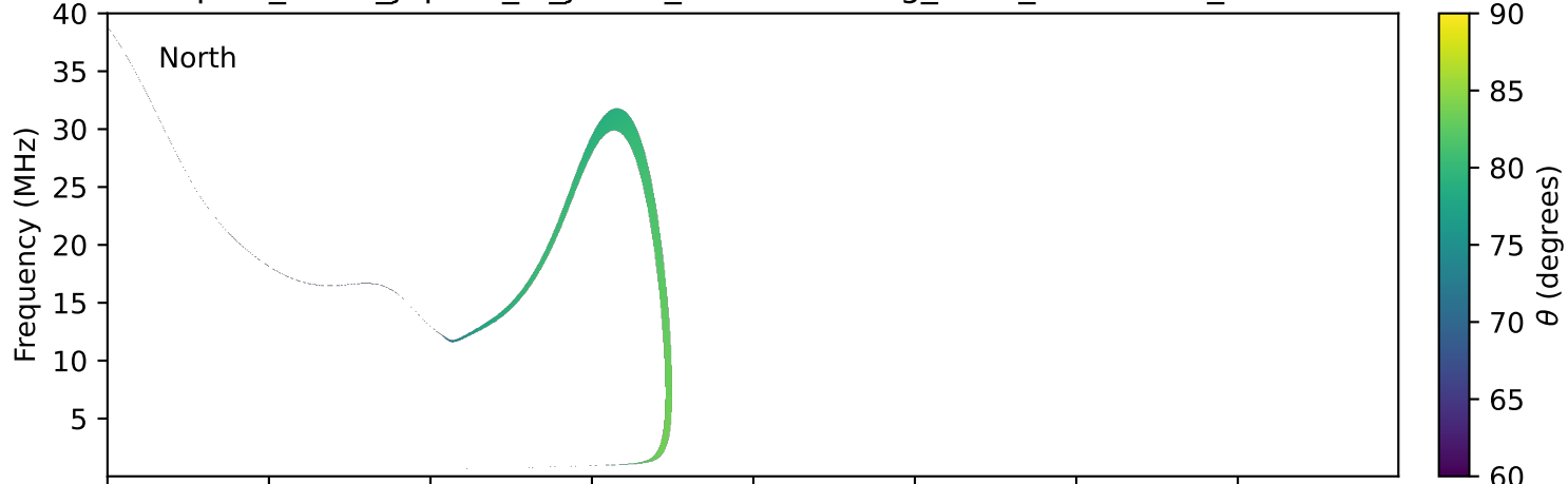
expres_earth_jupiter_io_jrm33_lossc-wid1deg_3kev_20000129_v11.cdf
