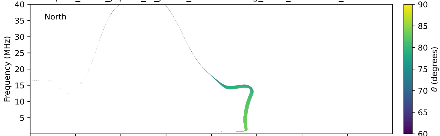
expres_earth_jupiter_io_jrm33_lossc-wid1deg_3kev_20000127_v11.cdf
