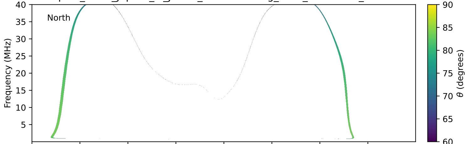
expres_earth_jupiter_io_jrm33_lossc-wid1deg_3kev_20000125_v11.cdf
