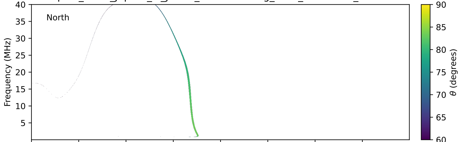
expres_earth_jupiter_io_jrm33_lossc-wid1deg_3kev_20000113_v11.cdf
