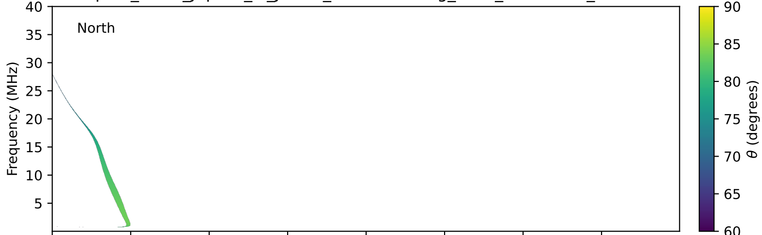
expres_earth_jupiter_io_jrm33_lossc-wid1deg_3kev_20000108_v11.cdf
