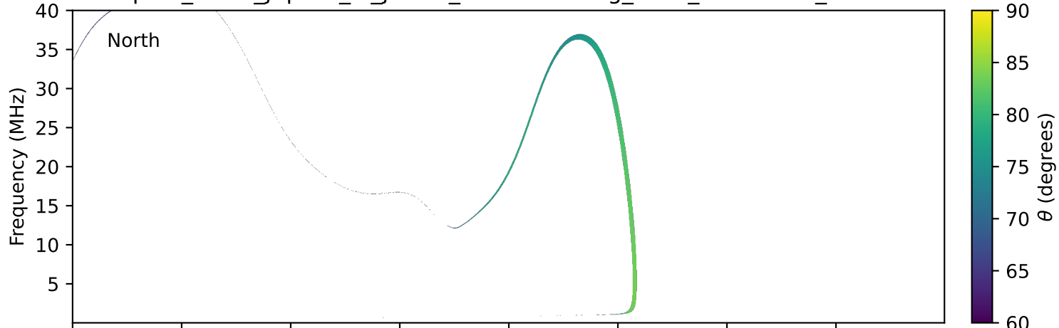
expres_earth_jupiter_io_jrm33_lossc-wid1deg_3kev_20000104_v11.cdf
