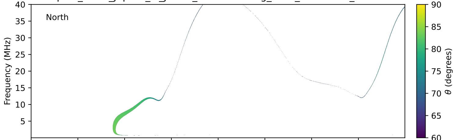
expres_earth_jupiter_io_jrm09_lossc-wid1deg_3kev_20000123_v11.cdf
