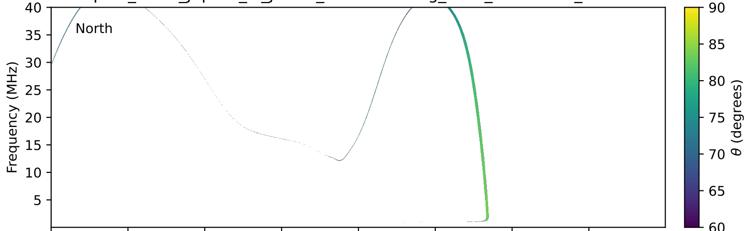
expres_earth_jupiter_io_jrm09_lossc-wid1deg_3kev_20000111_v11.cdf
