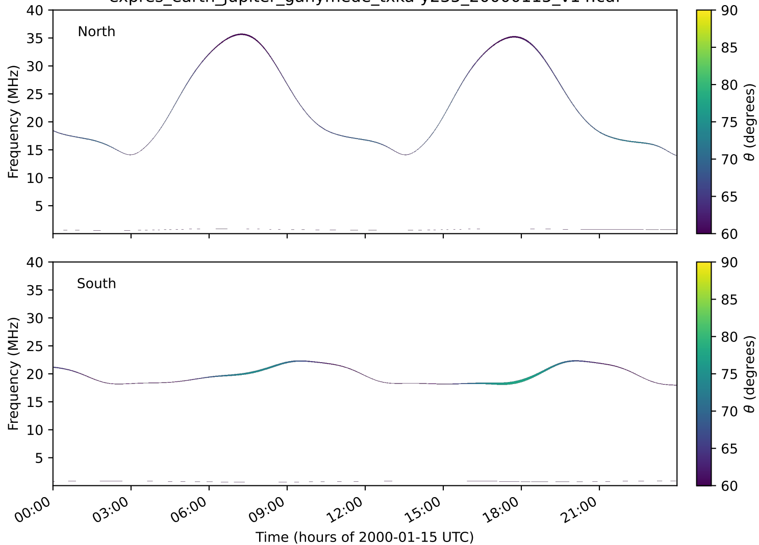
expres_earth_jupiter_ganymede_txka-y235_20000115_v14.cdf
