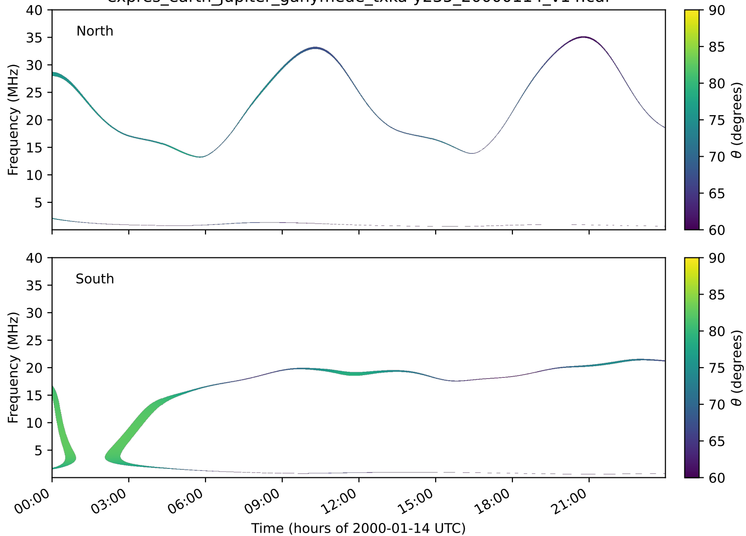
expres_earth_jupiter_ganymede_txka-y235_20000114_v14.cdf
