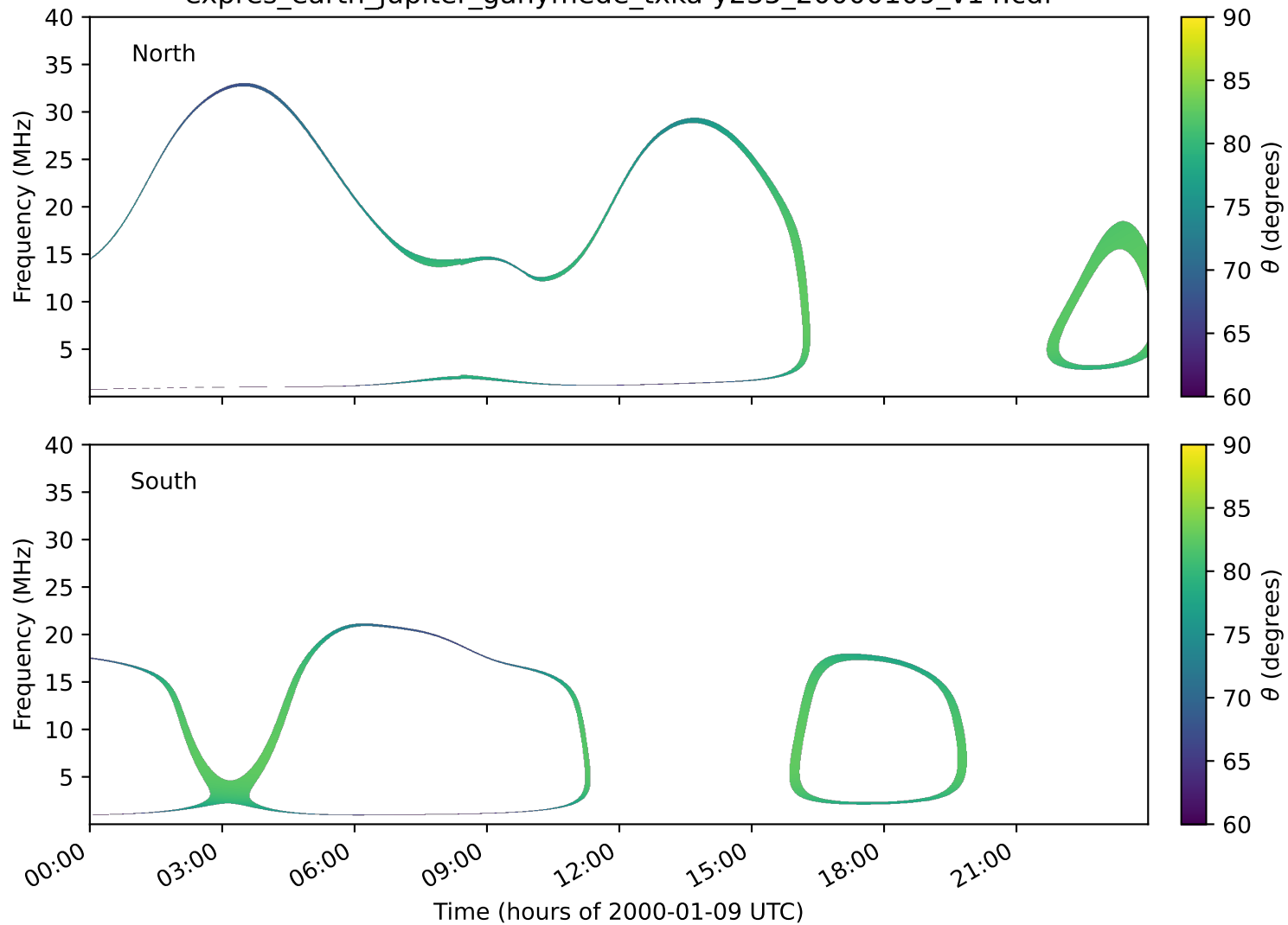
expres_earth_jupiter_ganymede_txka-y235_20000109_v14.cdf
