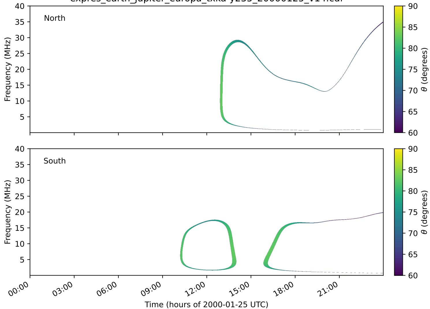
expres_earth_jupiter_europa_txka-y235_20000125_v14.cdf
