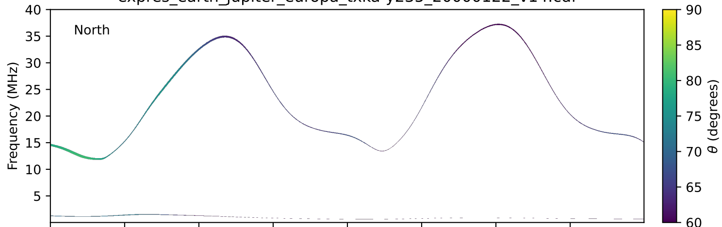
expres_earth_jupiter_europa_txka-y235_20000122_v14.cdf
