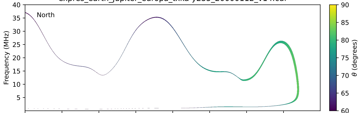
expres_earth_jupiter_europa_txka-y235_20000112_v14.cdf
