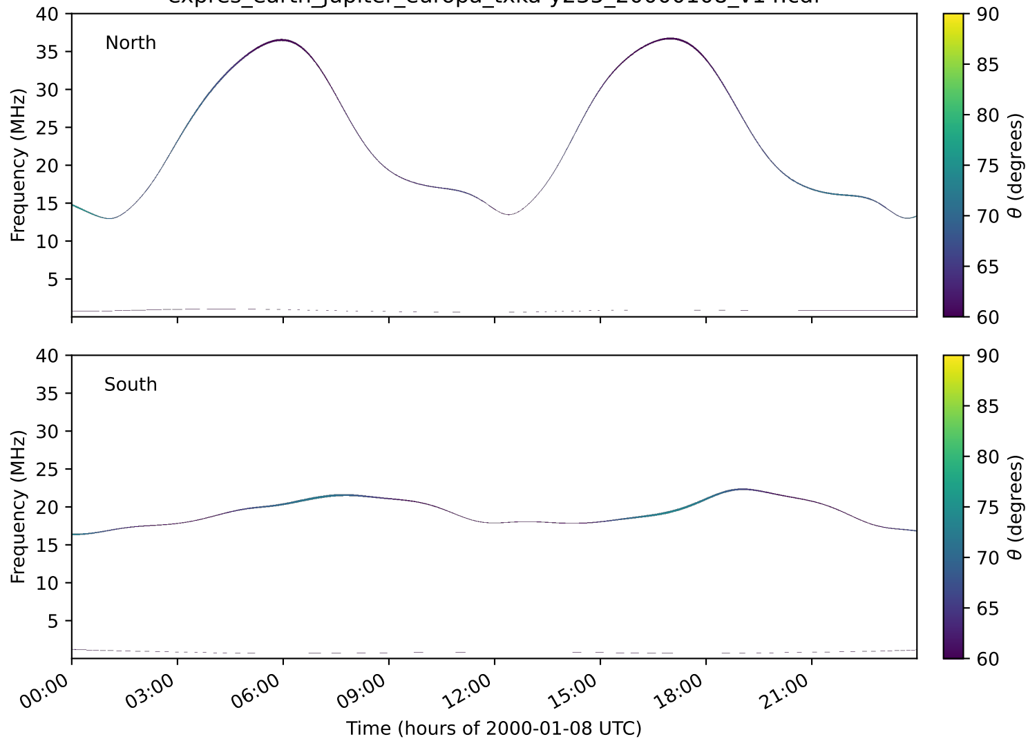
expres_earth_jupiter_europa_txka-y235_20000108_v14.cdf
