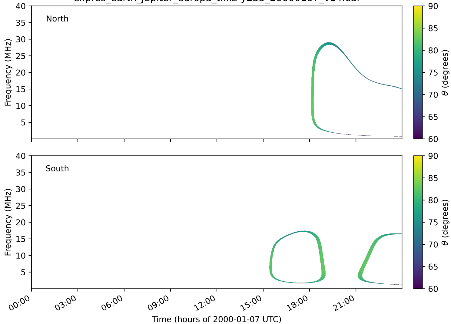
expres_earth_jupiter_europa_txka-y235_20000107_v14.cdf
