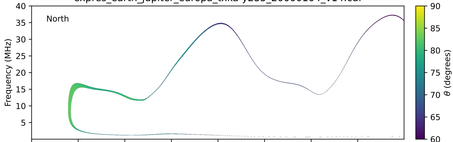
expres_earth_jupiter_europa_txka-y235_20000104_v14.cdf
