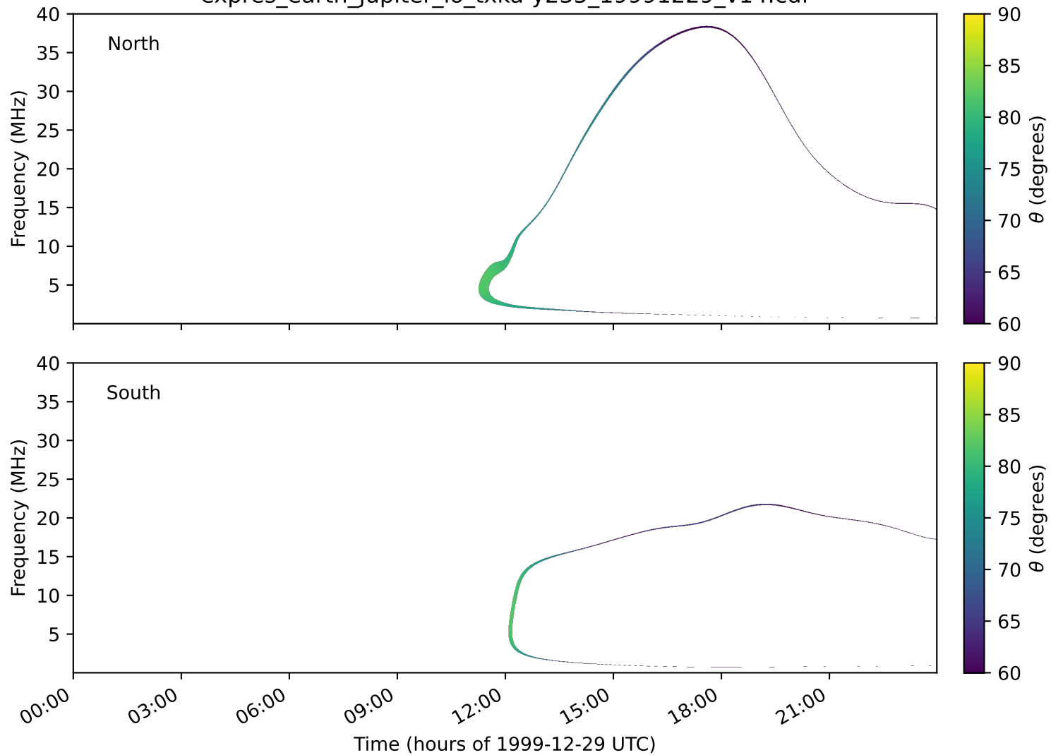
expres_earth_jupiter_io_txka-y235_19991229_v14.cdf
