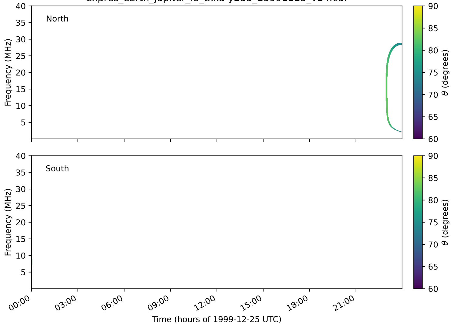
expres_earth_jupiter_io_txka-y235_19991225_v14.cdf
