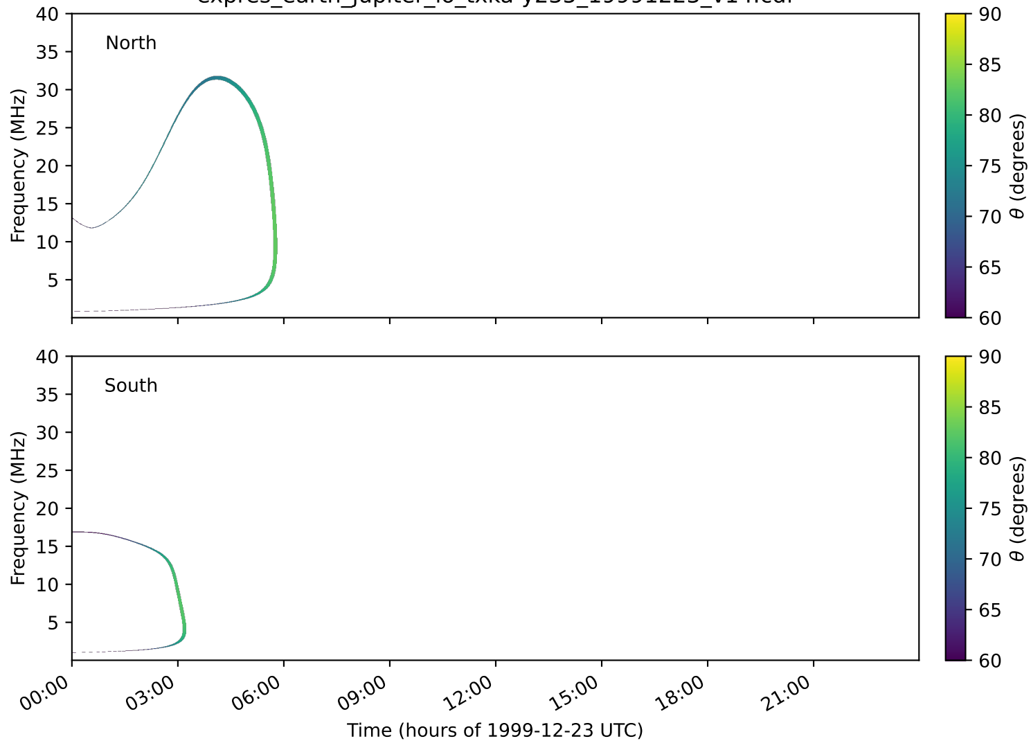
expres_earth_jupiter_io_txka-y235_19991223_v14.cdf
