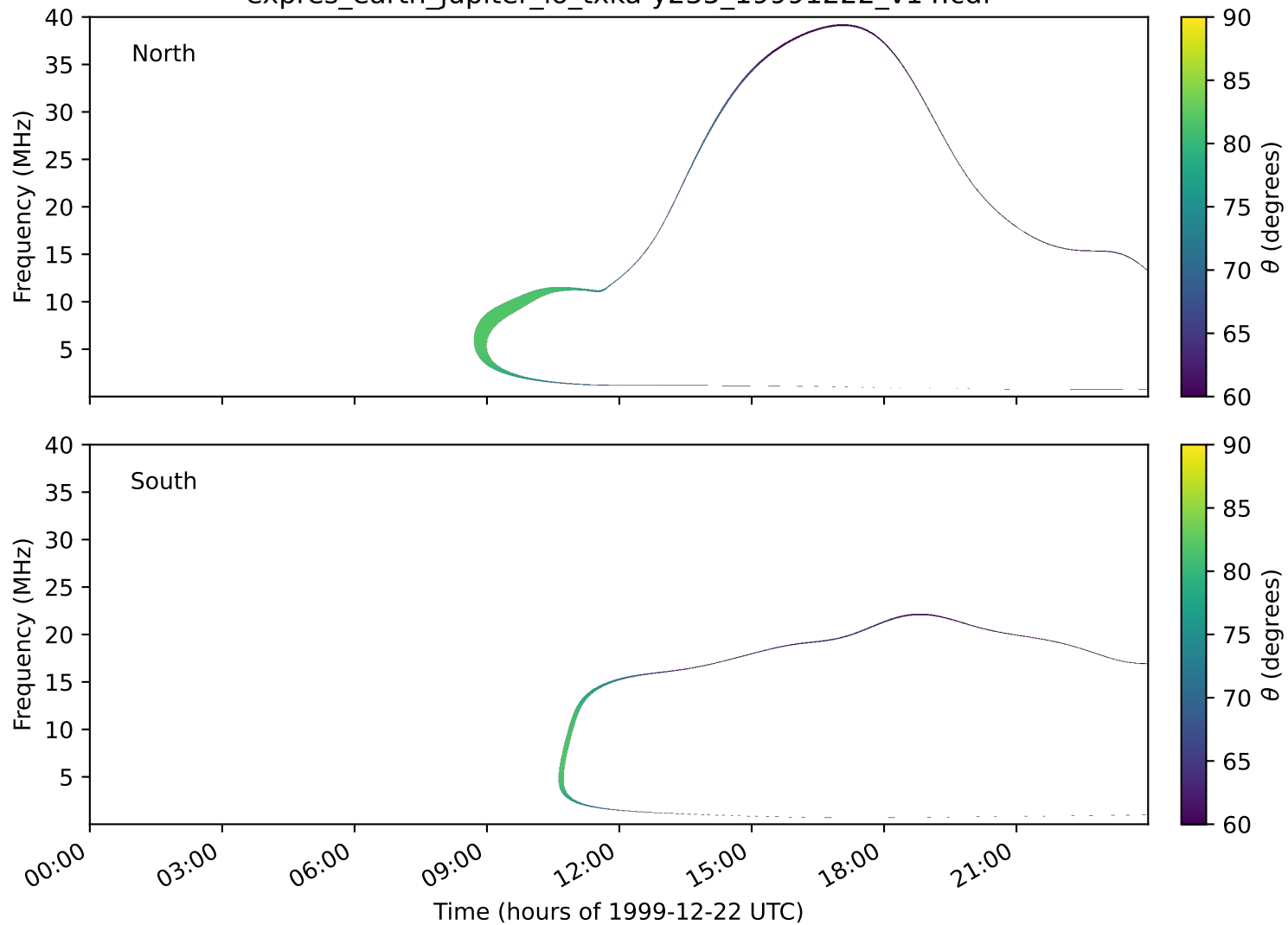
expres_earth_jupiter_io_txka-y235_19991222_v14.cdf
