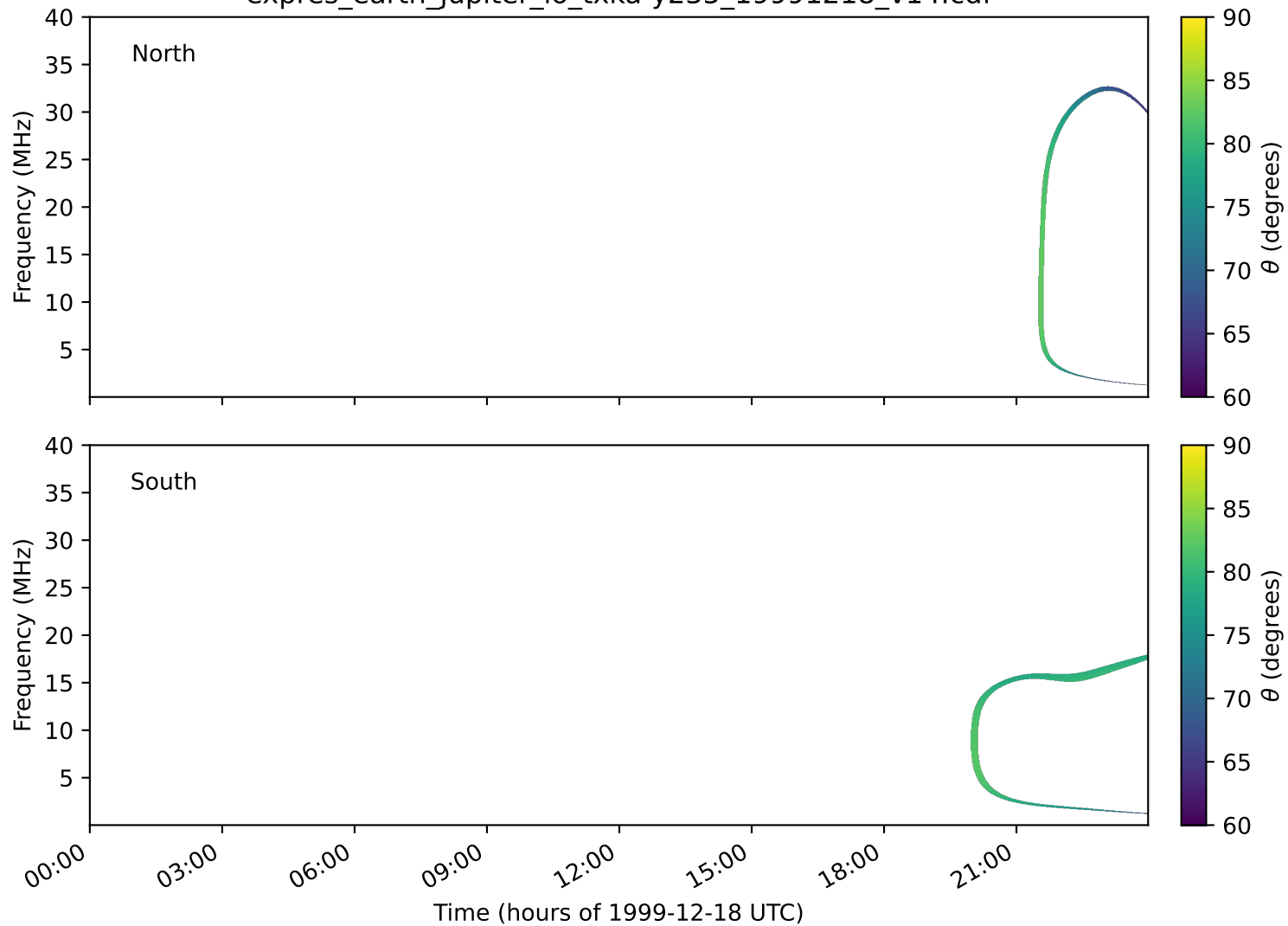
expres_earth_jupiter_io_txka-y235_19991218_v14.cdf
