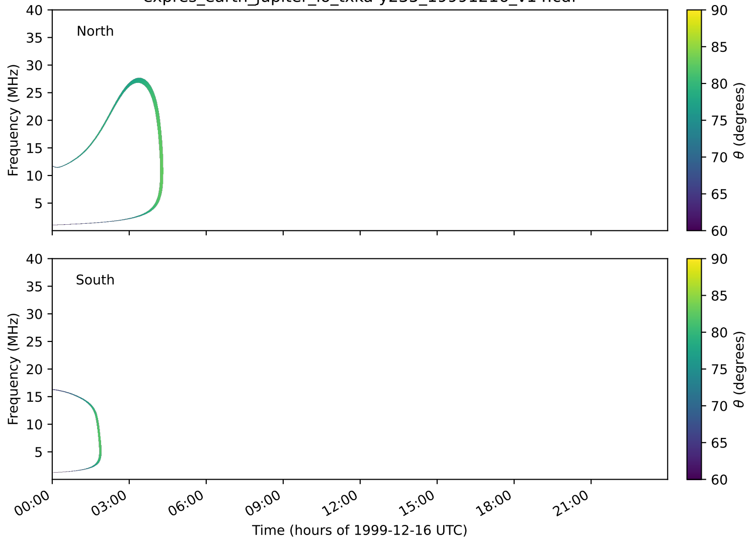
expres_earth_jupiter_io_txka-y235_19991216_v14.cdf
