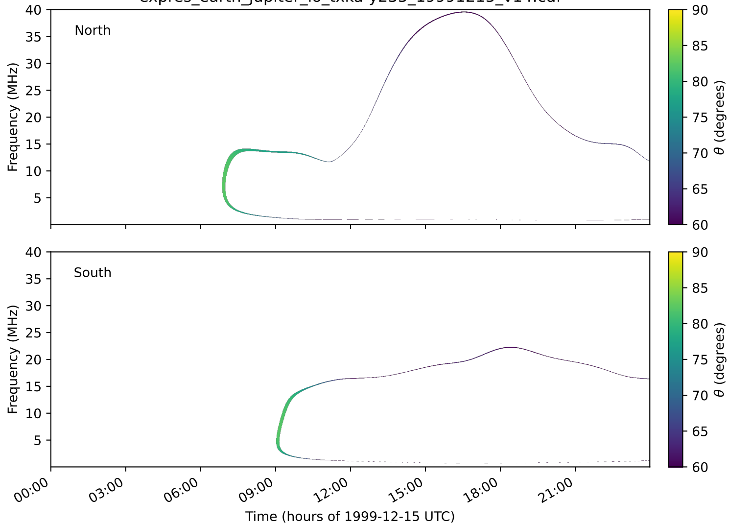
expres_earth_jupiter_io_txka-y235_19991215_v14.cdf
