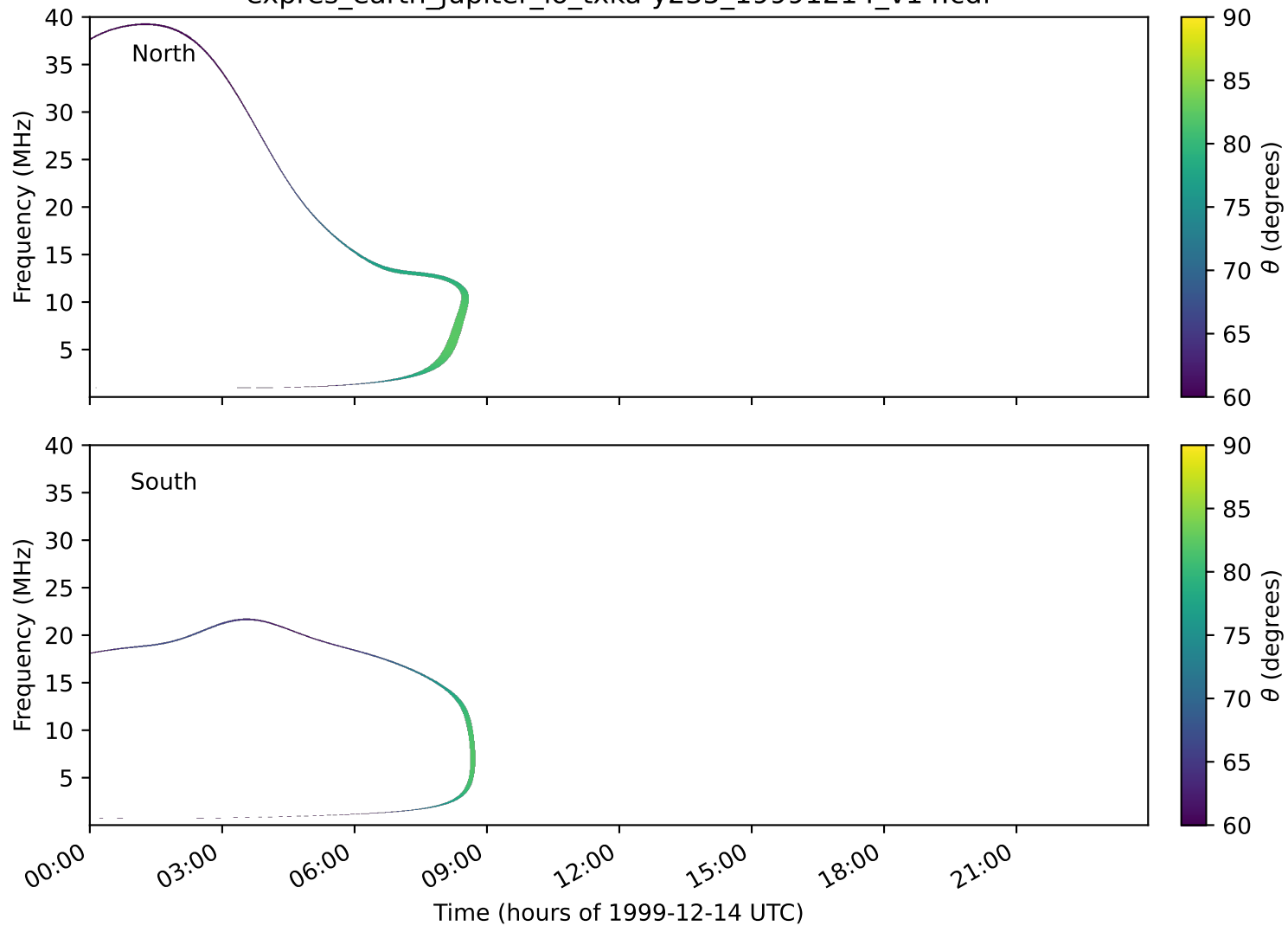
expres_earth_jupiter_io_txka-y235_19991214_v14.cdf
