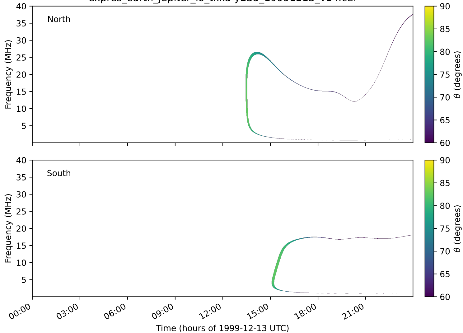
expres_earth_jupiter_io_txka-y235_19991213_v14.cdf
