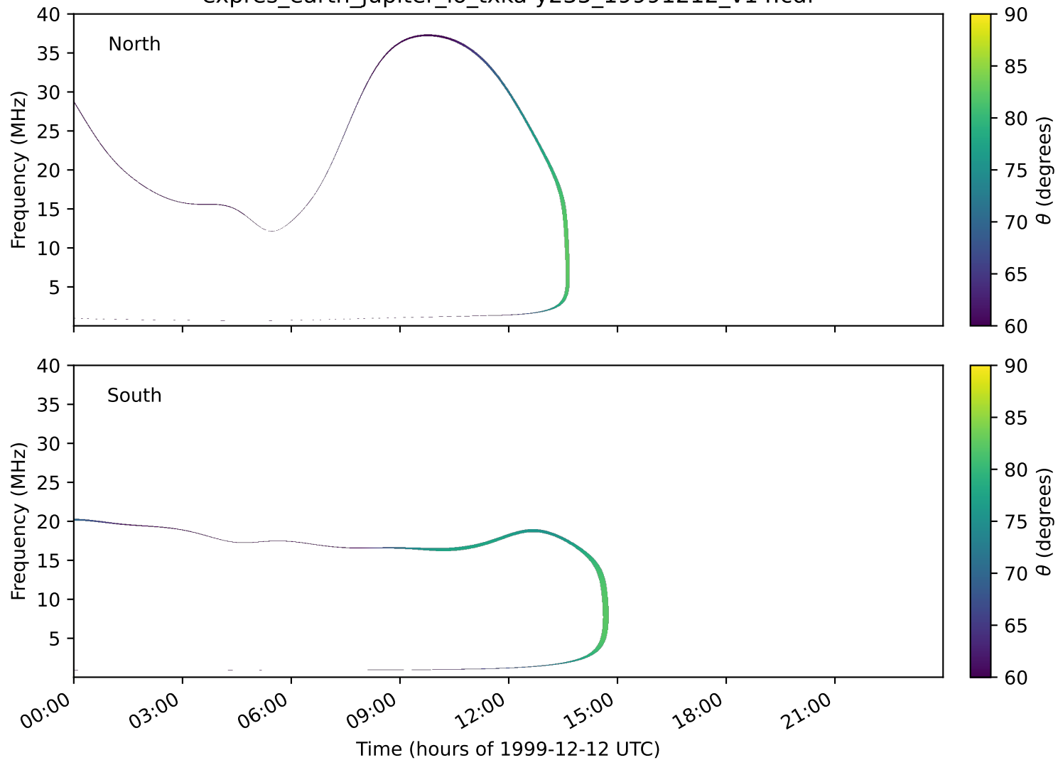
expres_earth_jupiter_io_txka-y235_19991212_v14.cdf
