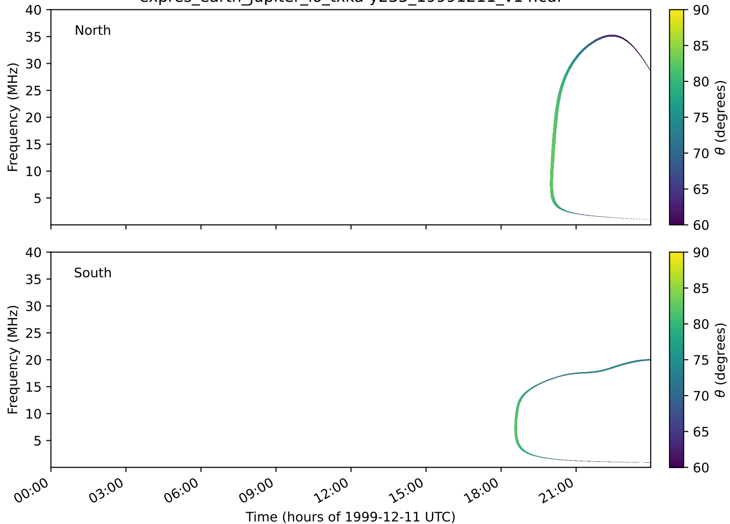
expres_earth_jupiter_io_txka-y235_19991211_v14.cdf
