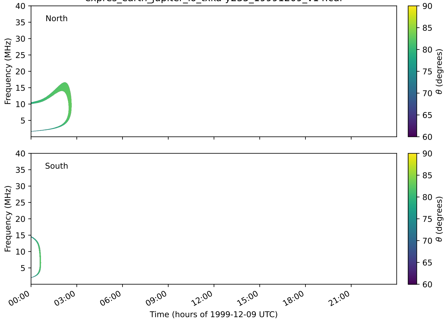
expres_earth_jupiter_io_txka-y235_19991209_v14.cdf
