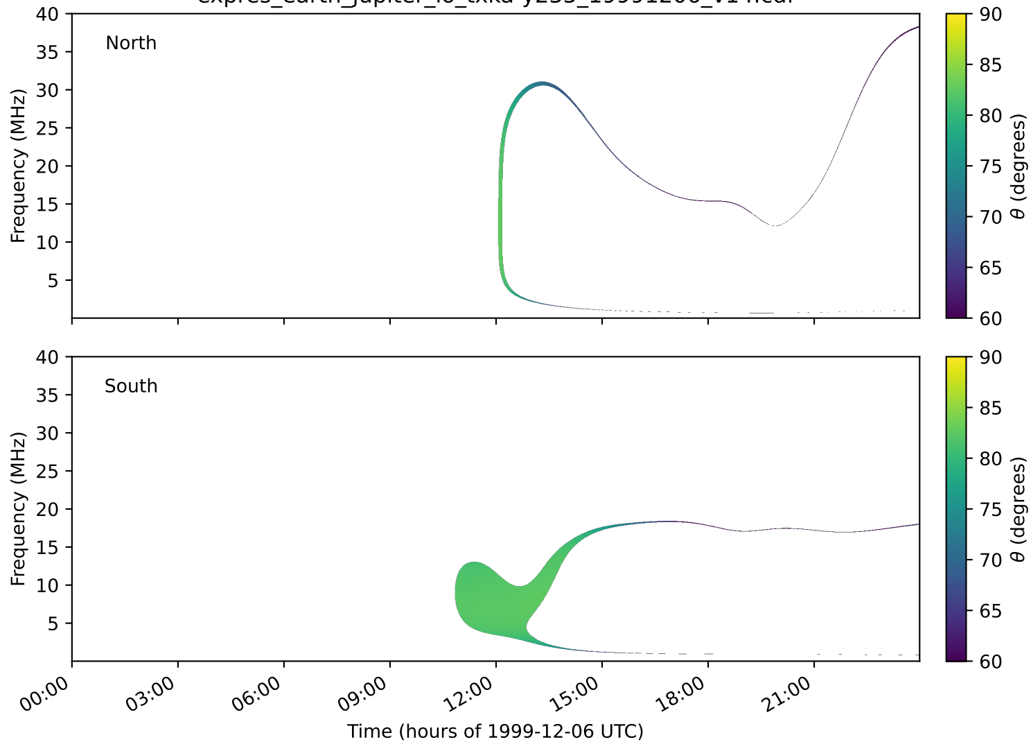
expres_earth_jupiter_io_txka-y235_19991206_v14.cdf
