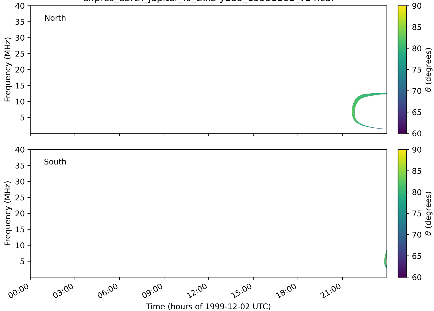
expres_earth_jupiter_io_txka-y235_19991202_v14.cdf
