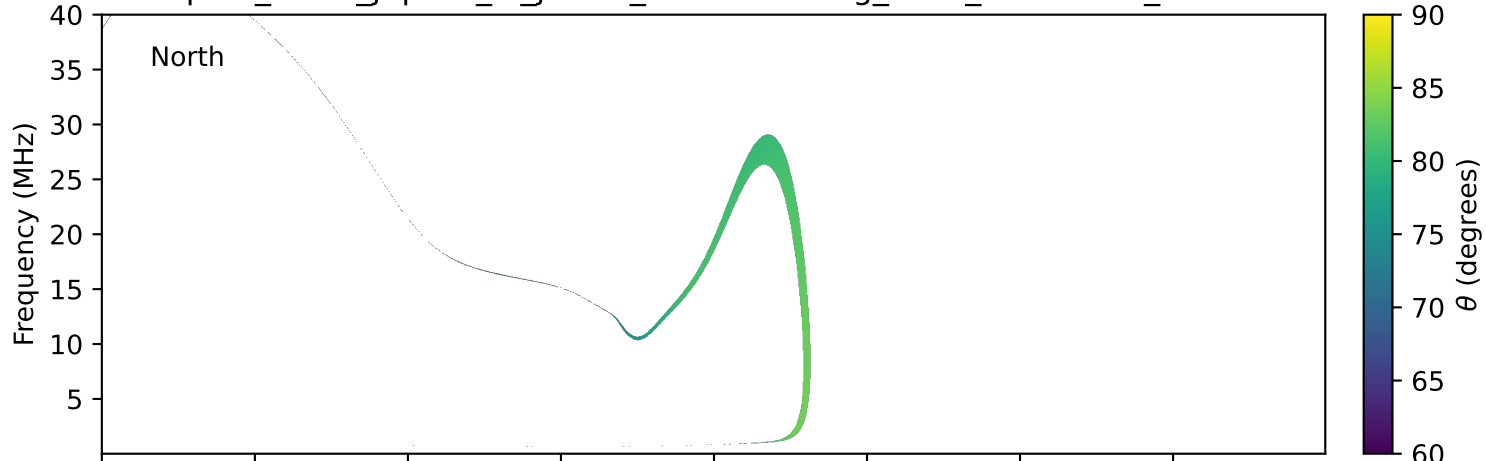
expres_earth_jupiter_io_jrm09_lossc-wid1deg_3kev_19991228_v11.cdf
