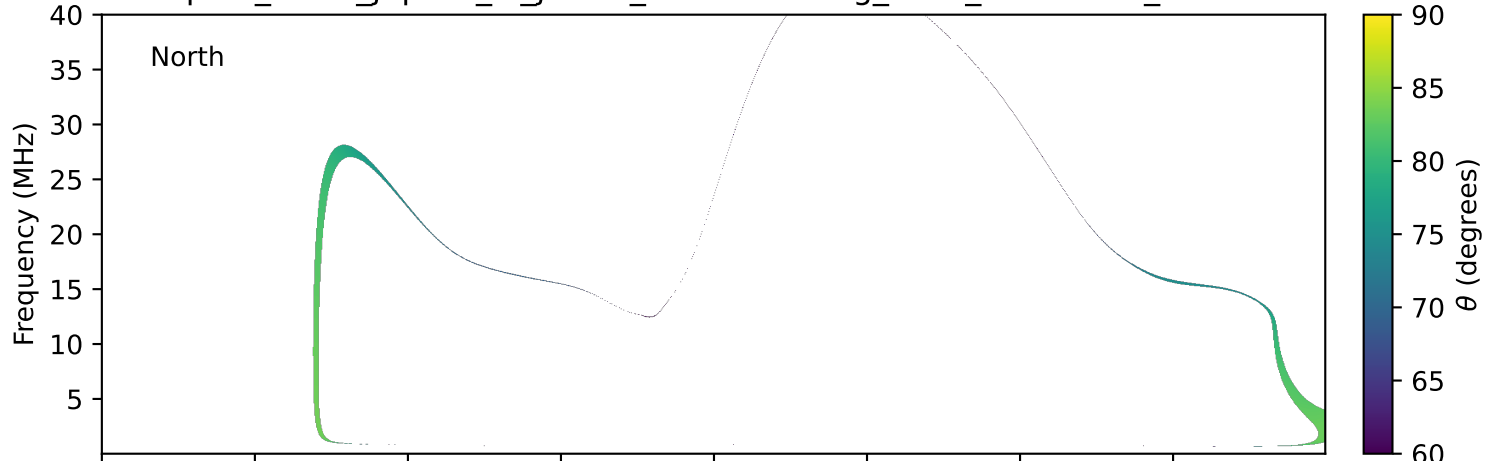
expres_earth_jupiter_io_jrm09_lossc-wid1deg_3kev_19991201_v11.cdf
