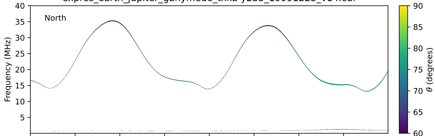
expres_earth_jupiter_ganymede_txka-y235_19991225_v14.cdf
