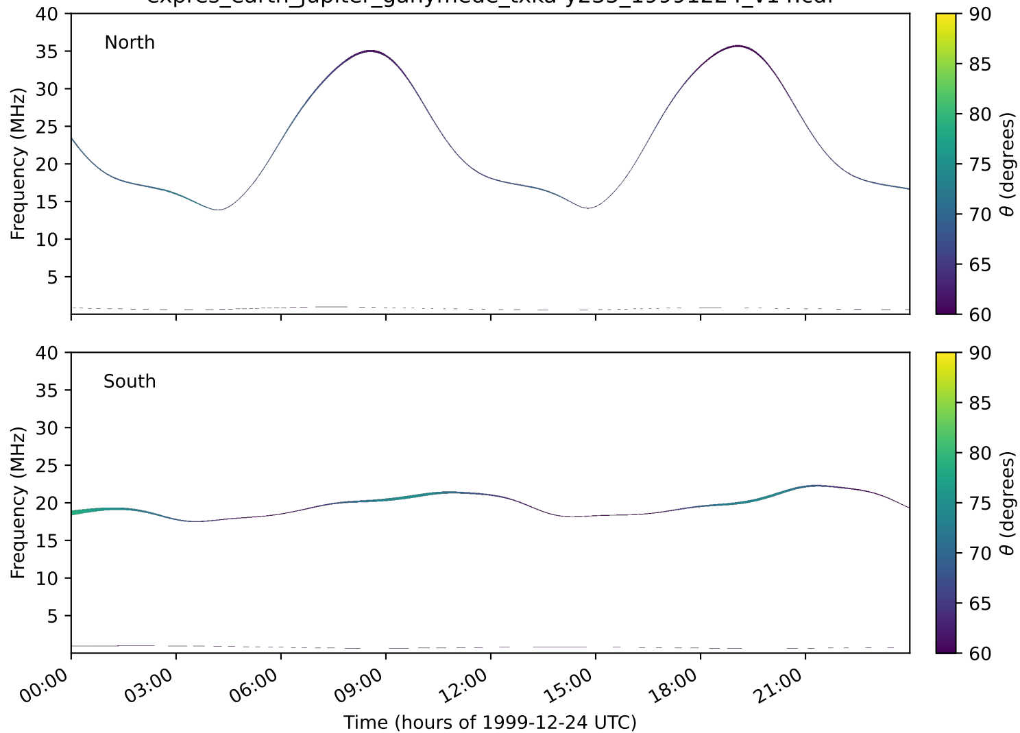
expres_earth_jupiter_ganymede_txka-y235_19991224_v14.cdf
