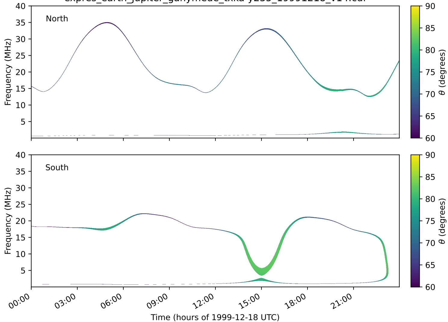
expres_earth_jupiter_ganymede_txka-y235_19991218_v14.cdf
