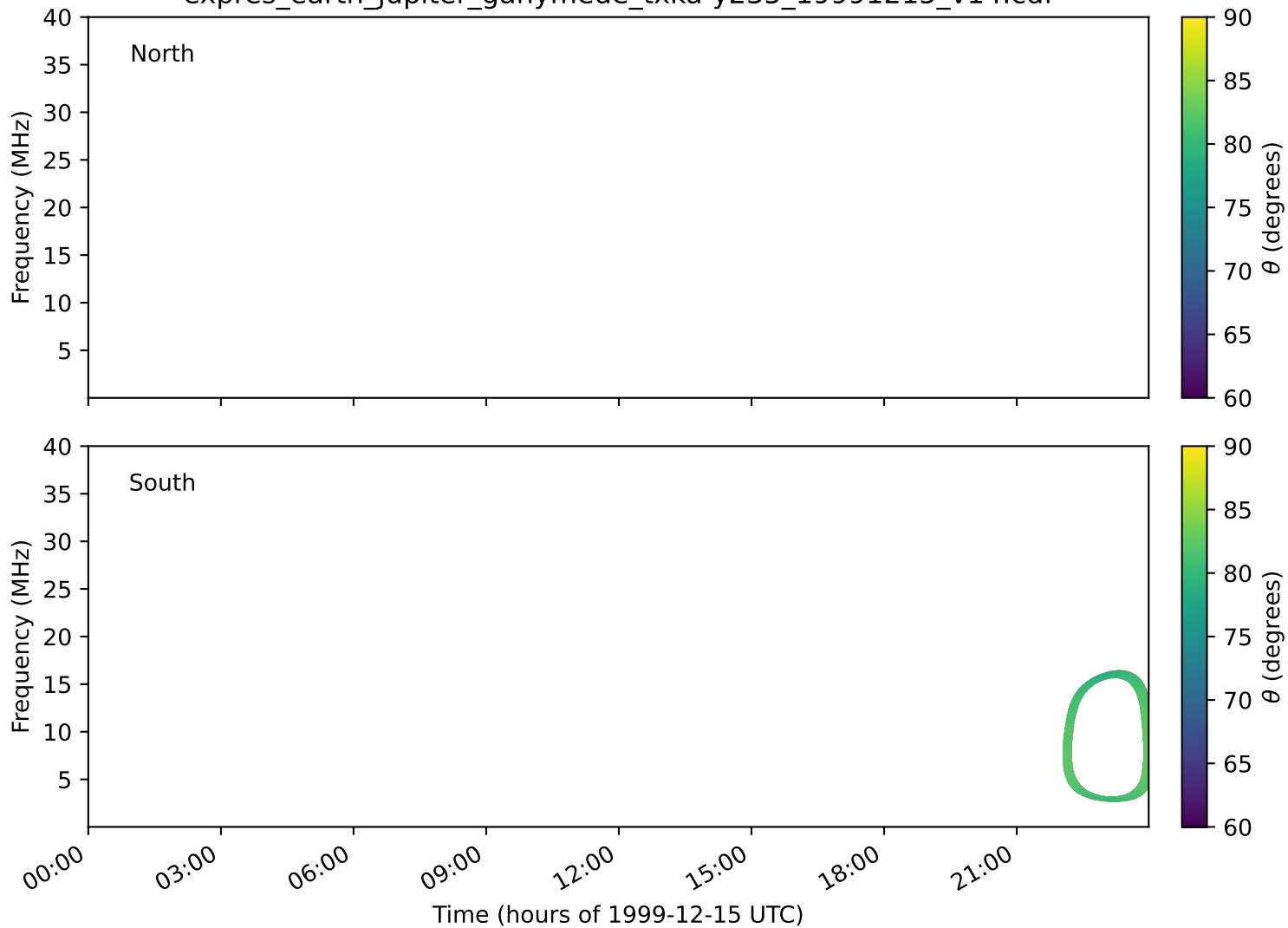
expres_earth_jupiter_ganymede_txka-y235_19991215_v14.cdf
