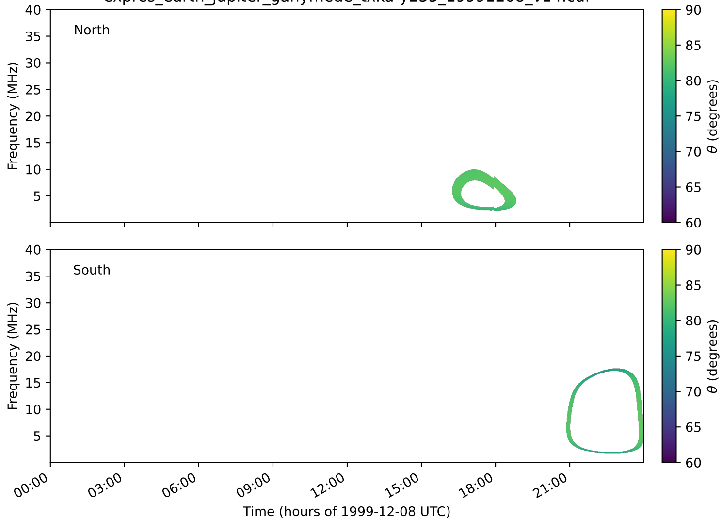
expres_earth_jupiter_ganymede_txka-y235_19991208_v14.cdf
