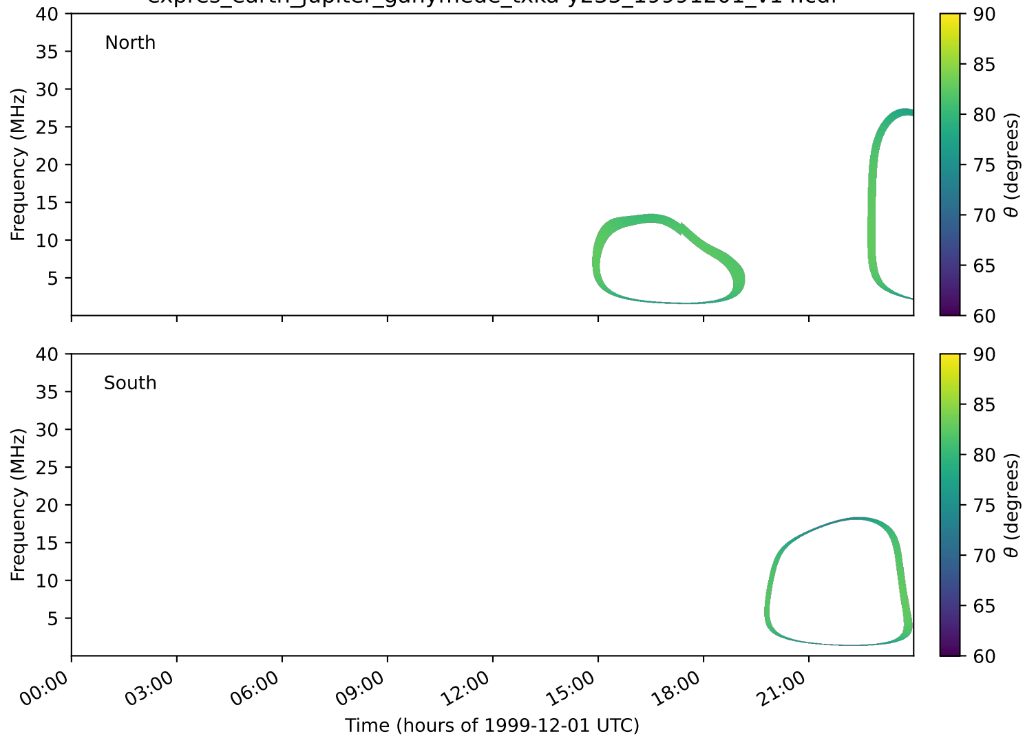
expres_earth_jupiter_ganymede_txka-y235_19991201_v14.cdf
