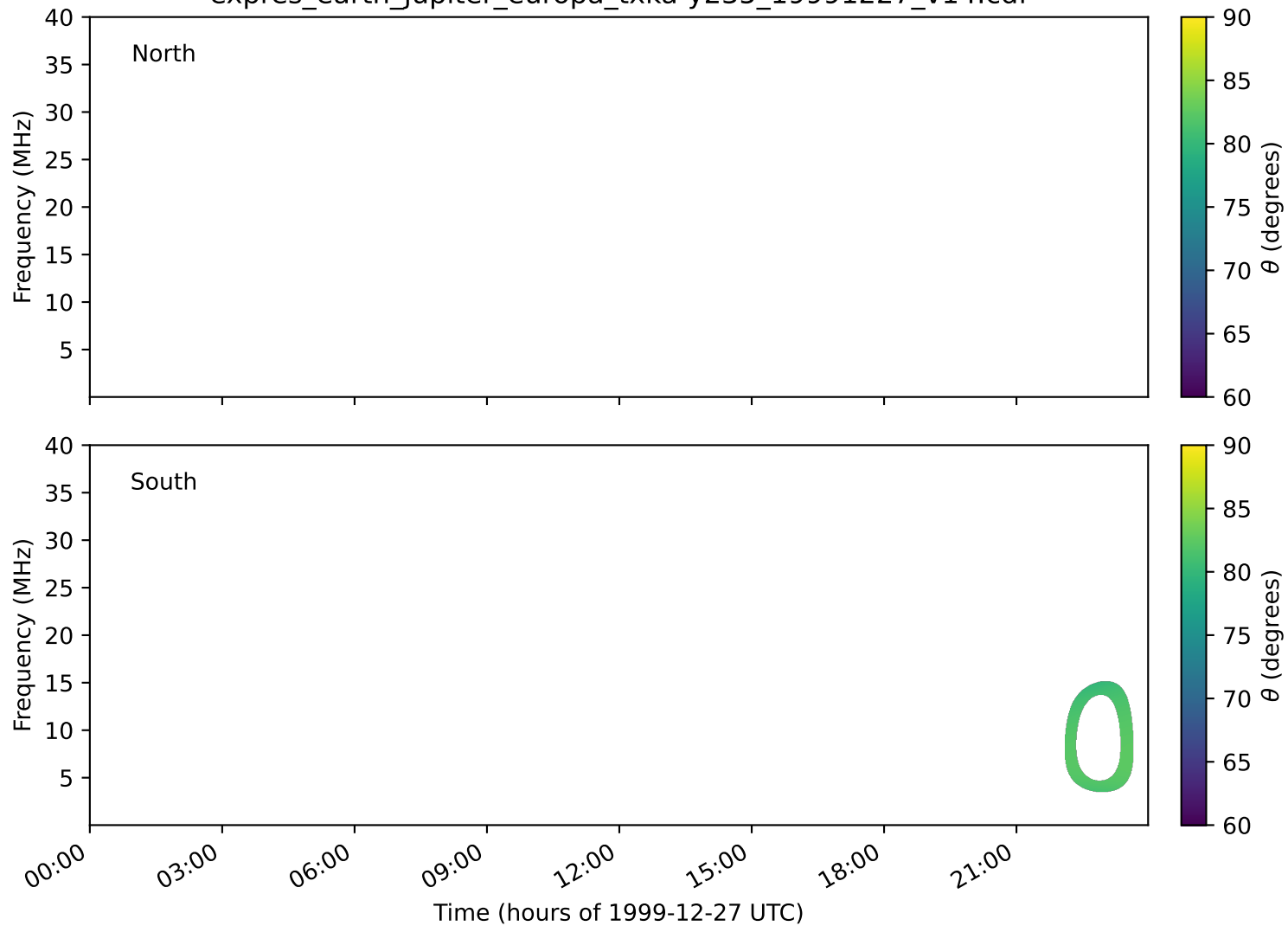
expres_earth_jupiter_europa_txka-y235_19991227_v14.cdf
