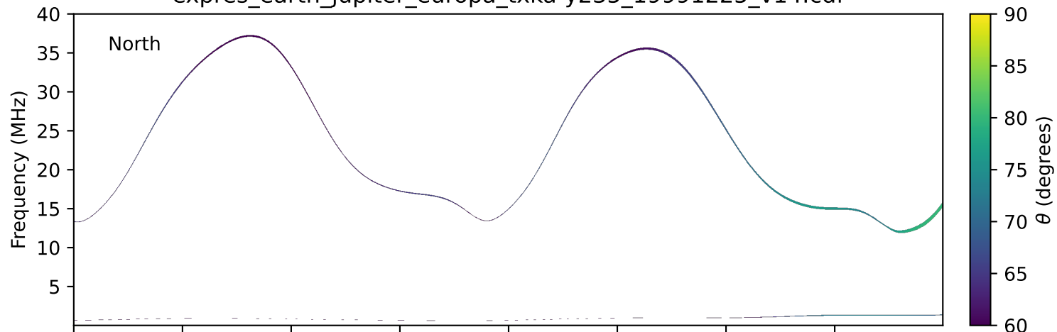
expres_earth_jupiter_europa_txka-y235_19991225_v14.cdf
