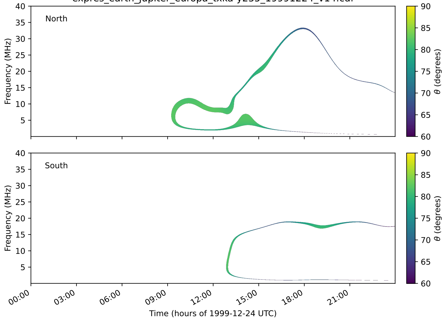
expres_earth_jupiter_europa_txka-y235_19991224_v14.cdf
